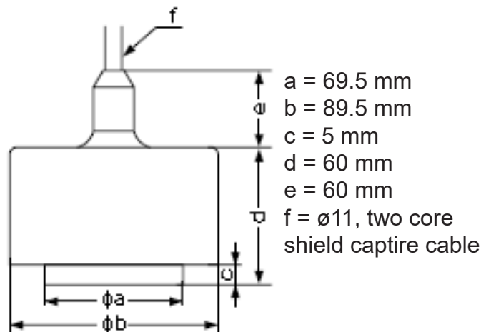
Dimensions of transducer without adaptor
